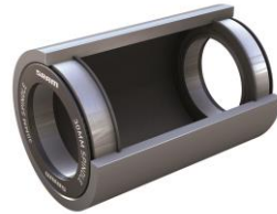
BB30 (aksel \varnothing 30 mm)
